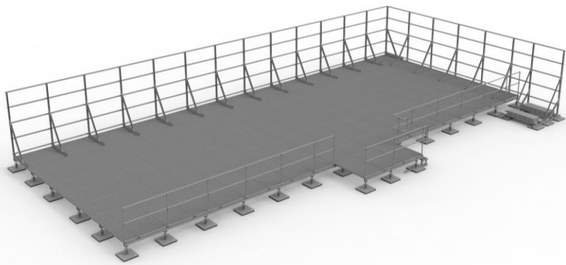
PLANTDECK WITH LOUVRE SYSTEM
